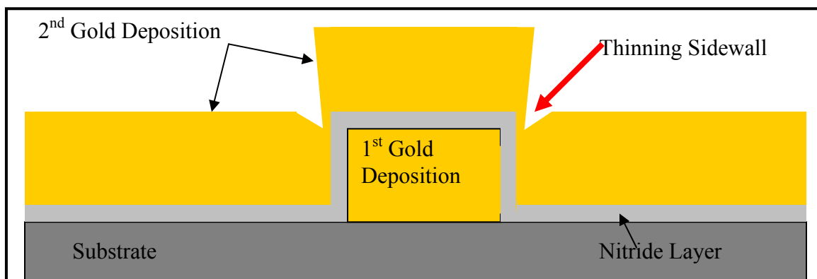
Figure 7.1: Potential thinning sidewalls created as a result of metal deposition method.
