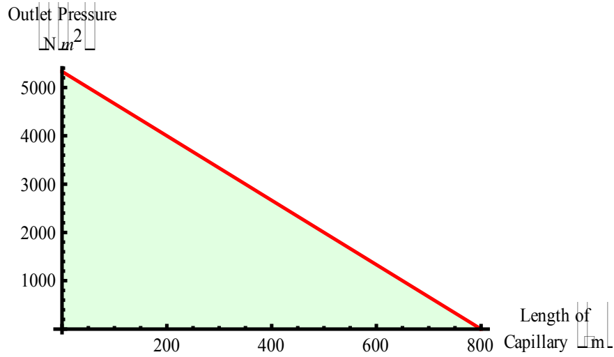
Figure 4.1: Fluid pressure in the microchannel as a function of channel length. Pressure at the channel inlet is 5332.9 \text{ N/m}^2 .
